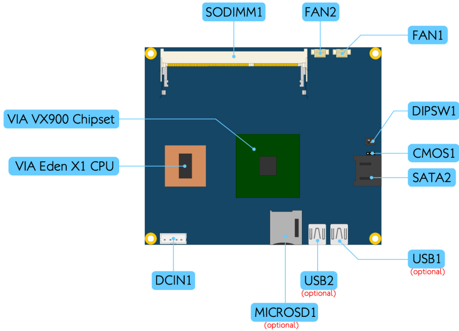
Figure 1: Layout diagram of the VIA ETX-8X90-10GR module (top side)
