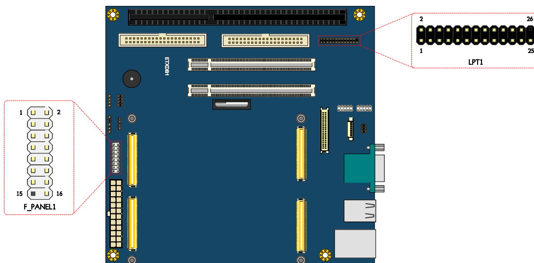
Figure 48: Front panel and LPT pin headers diagram
